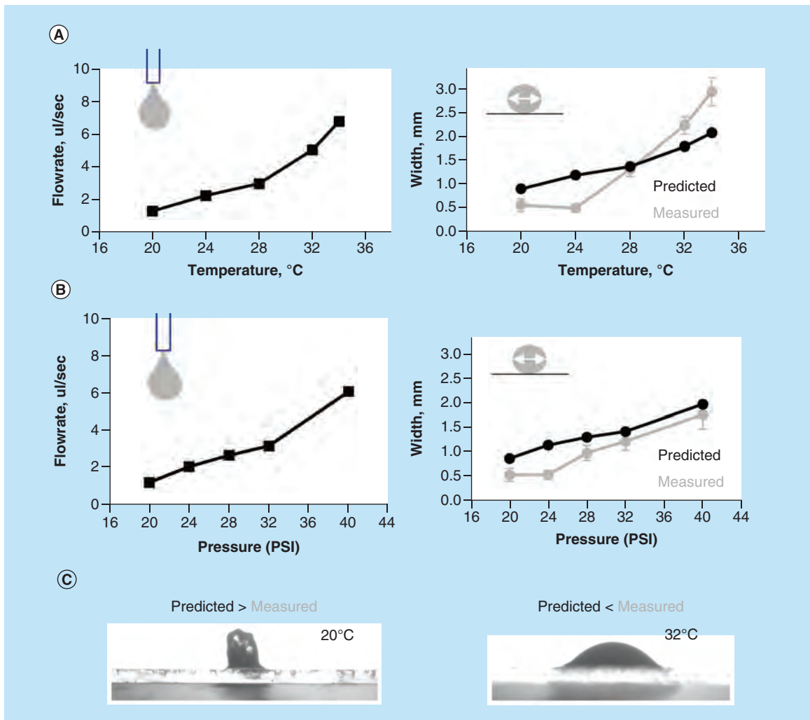
Figure 2. Effects of extrusion pressure and temperature on width of printed gelatin methacryloyl struts. (A) Predicted versus measured width of GelMA struts. Left panel: the flowrate of 15% GelMA printed using 23-gauge needle at specified temperatures was determined based on the weight of extruded hydrogel. Right panel: thickness of printed lines was then measured experimentally (grey symbols) and compared with the predicted thickness of cylindrically shaped struts (black symbols) based on flowrate values shown in A. Temperature above 28°C led to a wider than predicted struts, while temperature below led to a more narrow ones. (B) Similar measurements done at a constant temperature of 20°C while altering extruder pressure values. (C) Illustrative cross-sections of struts printed at 20° and 32°C are shown. GelMA: Gelatin methacryloyl.
